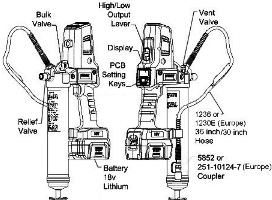
Figure 1 (1860 Grease Gun)
